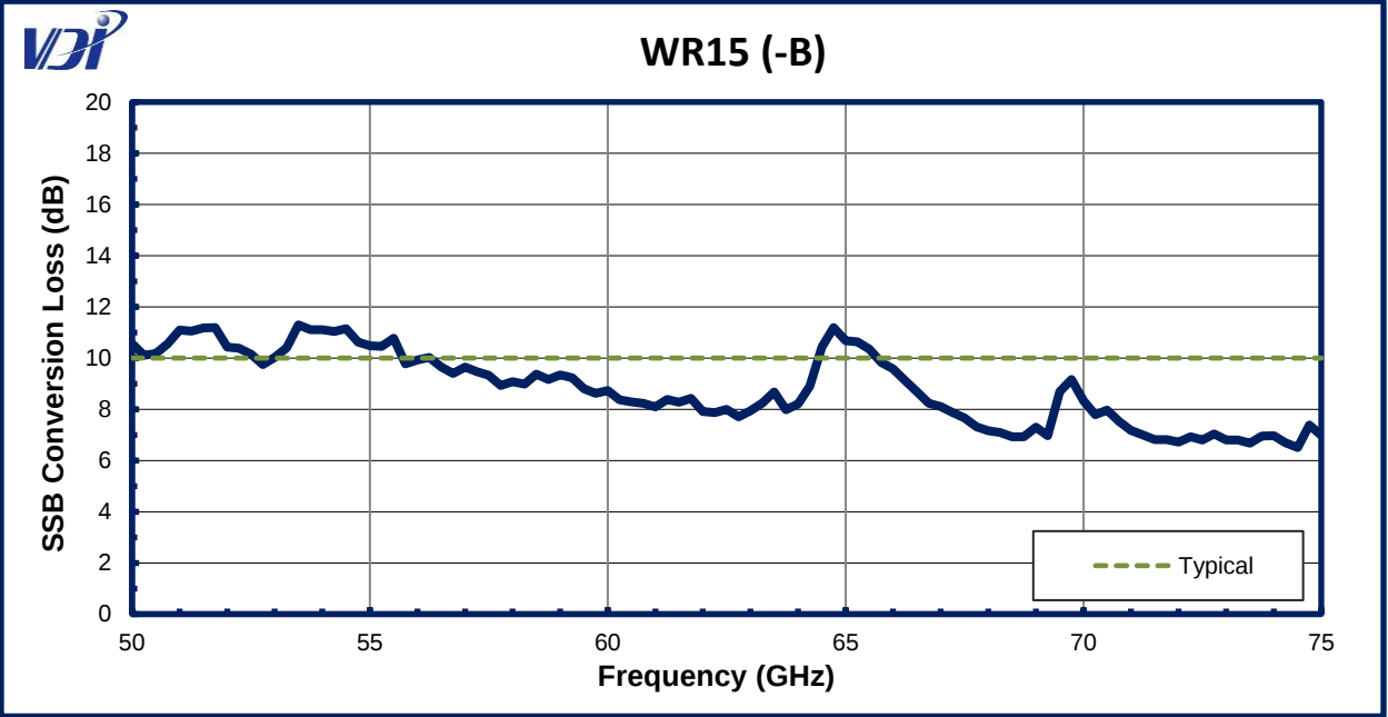
CCU/CCD Single Side Band (SSB) Conversion Loss Performance - continued
